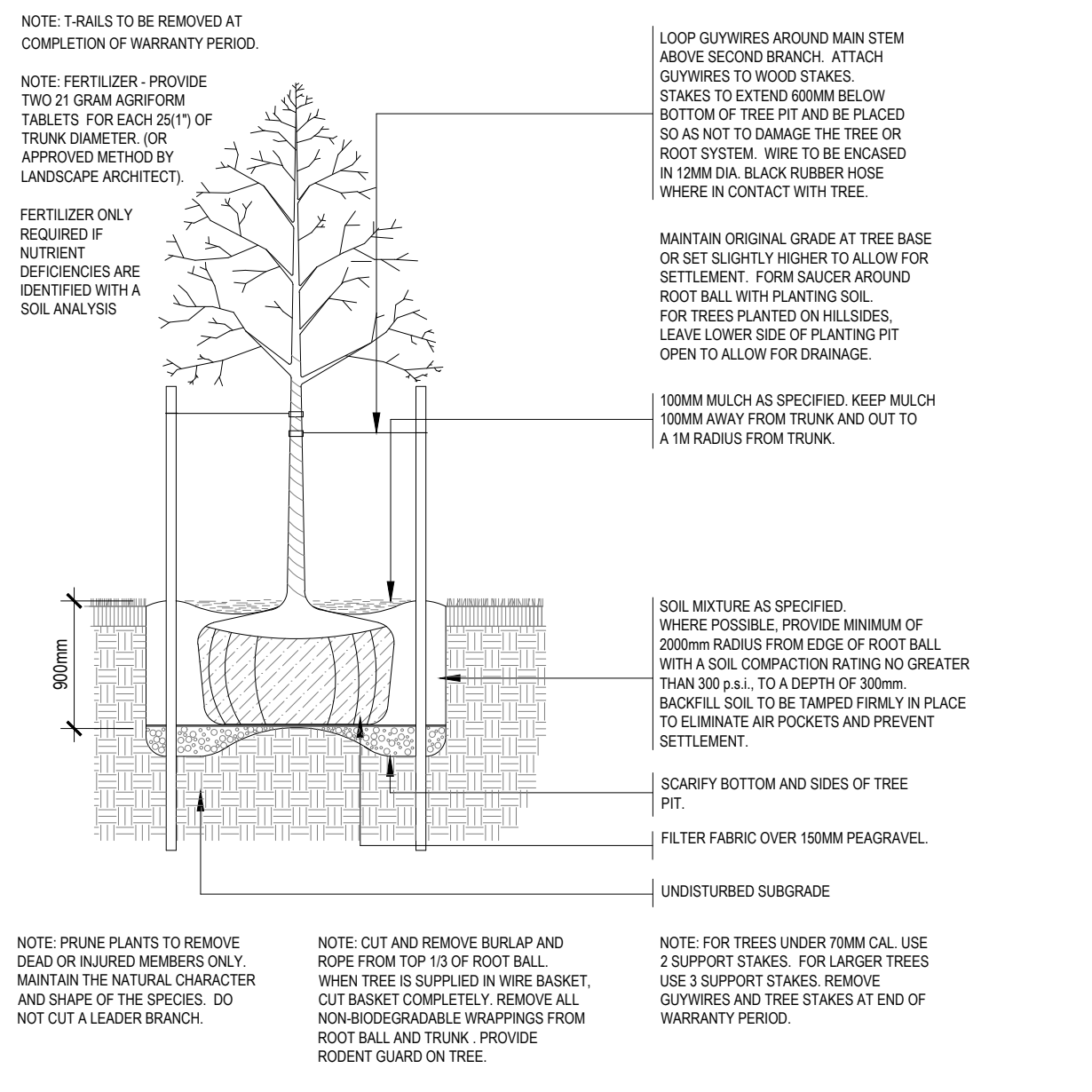
2 DECIDUOUS TREE PLANTING DETAIL L-2 N.T.S.
